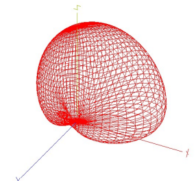
1/2\lambda Beverages RDF 8.11 dB 50-deg -3dB
