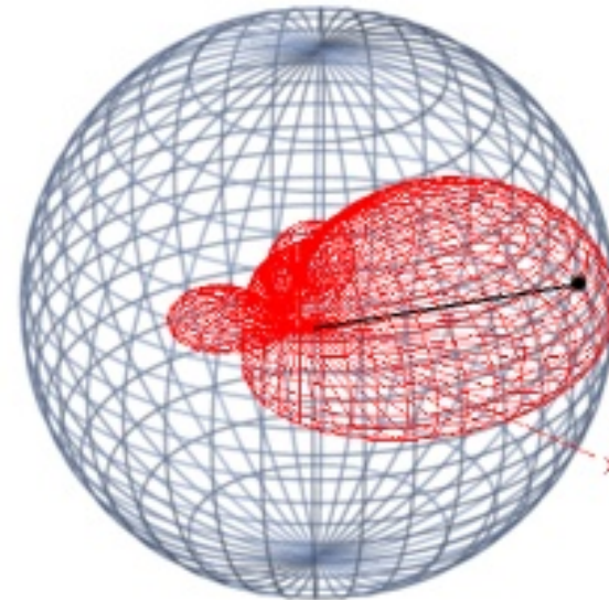
Four Square Array ( reduced power vs. vertical )
