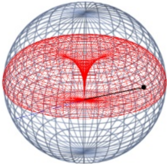
Omni-directional Vertical
