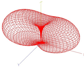
Verticals RDF 8.3 dB 60-deg -3dB Bi-directional
